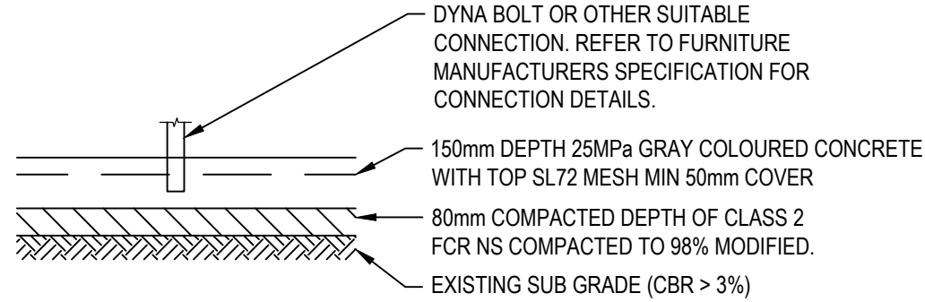
FURNITURE FOOTING DETAIL SCALE 1:20
