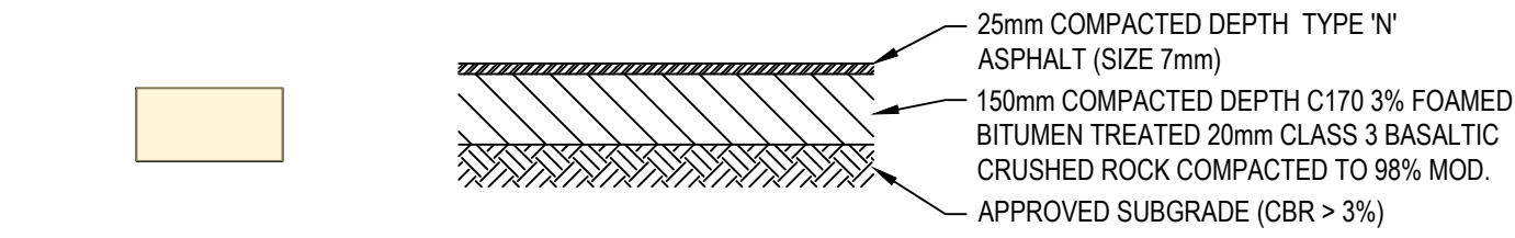
VEHICLE AND PEDESTRIAN ASPHALT PAVEMENT SCALE 1:20
